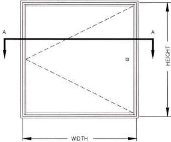
FRONT ELEVATION NOT TO SCALE
