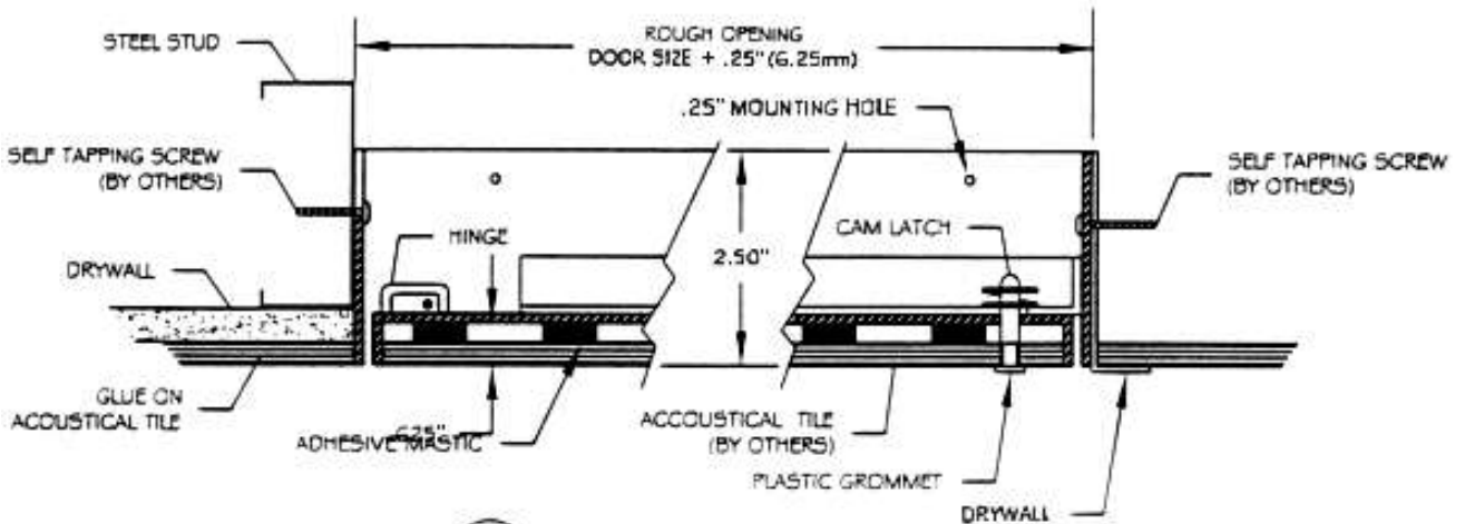
A CUT-THRU SECTION A NOT TO SCALE
